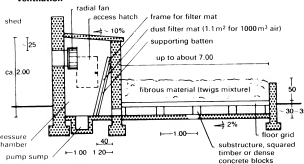
8 Earth filter system (design according to Zeisig)
